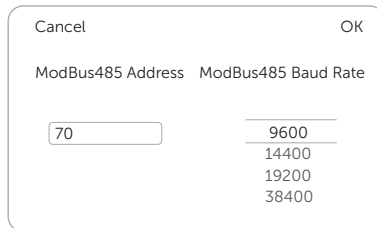
Figure 10-17 Modbus setting
